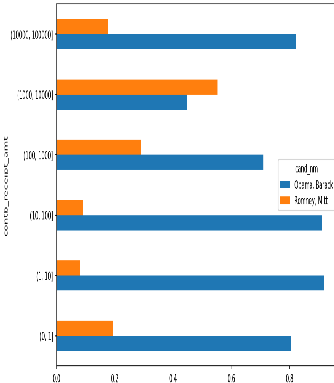
Figure 14-13. Percentage of total donations received by candidates for each donation size
