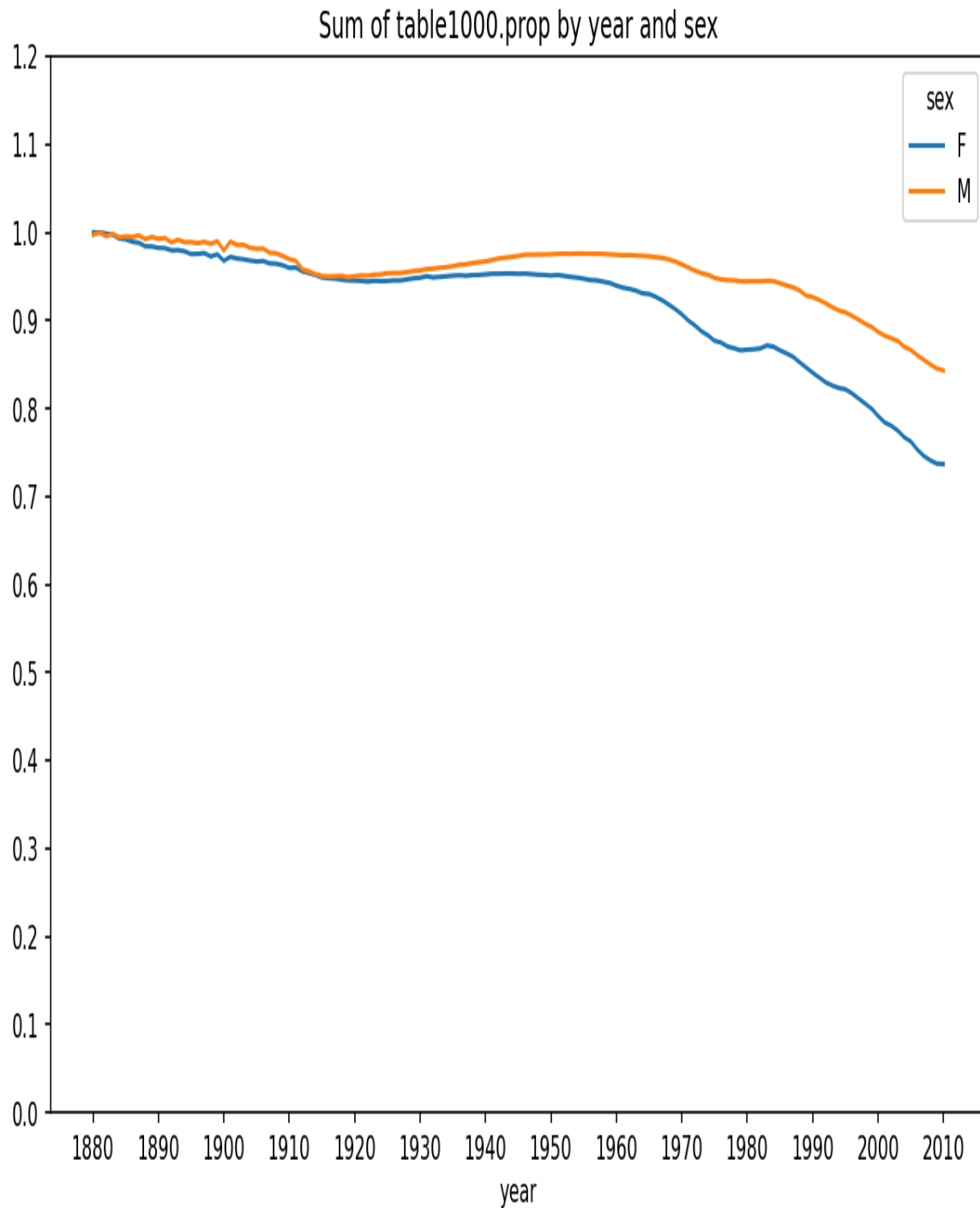
Figure 14-6. Proportion of births represented in top 1000 names by sex
