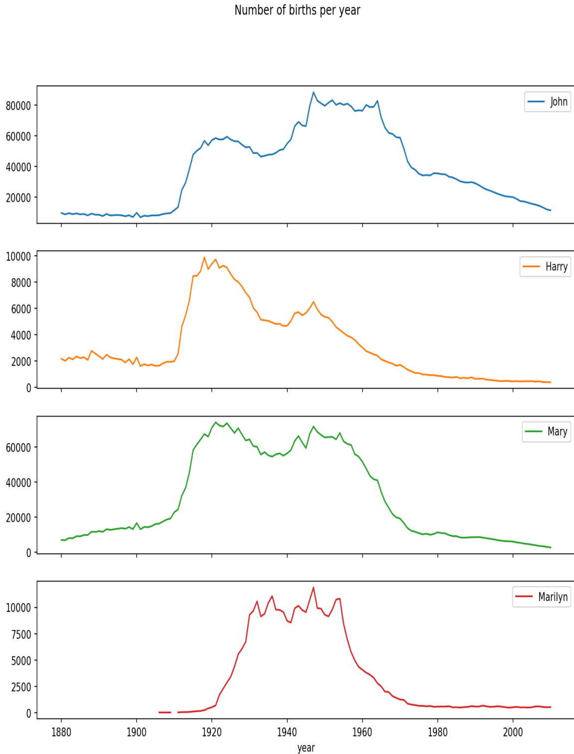
Figure 14-5. A few boy and girl names over time
