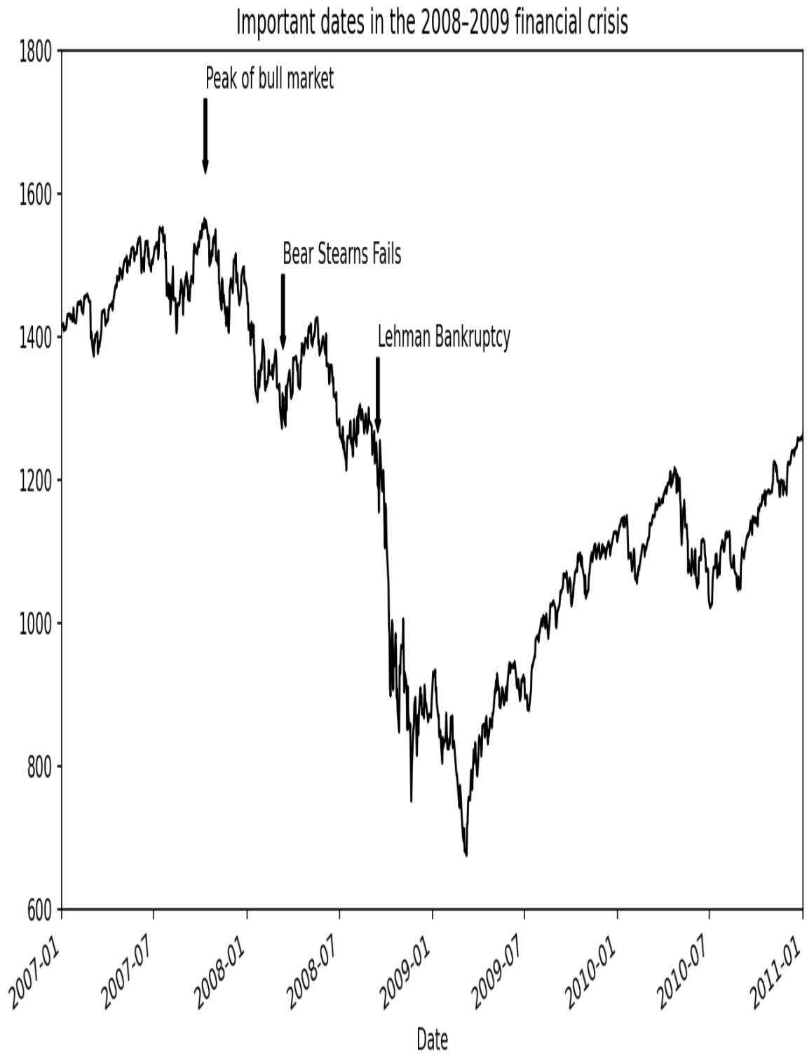
Figure 9-11. Important dates in the 2008–2009 financial crisis
