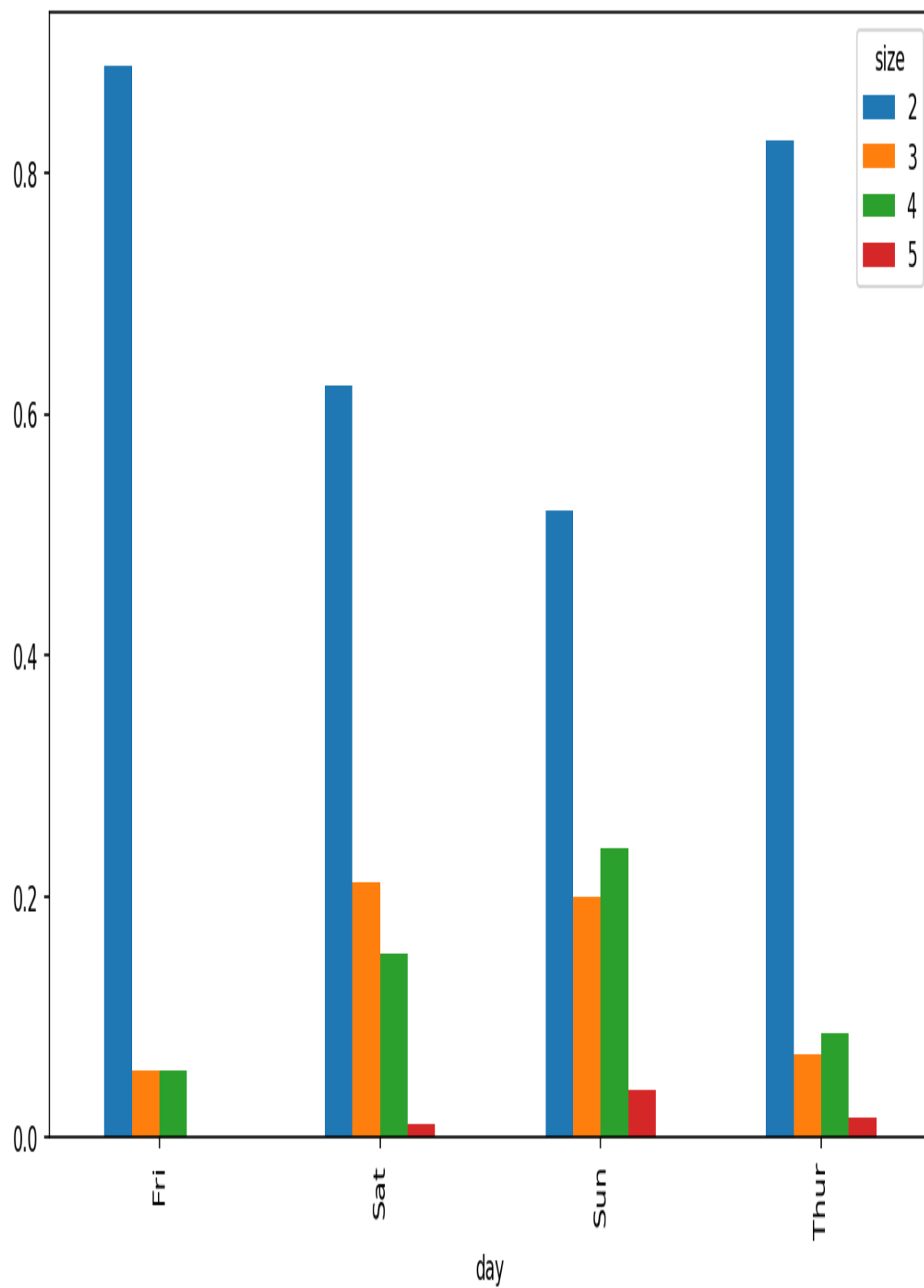
Figure 9-18. Fraction of parties by size within each day
