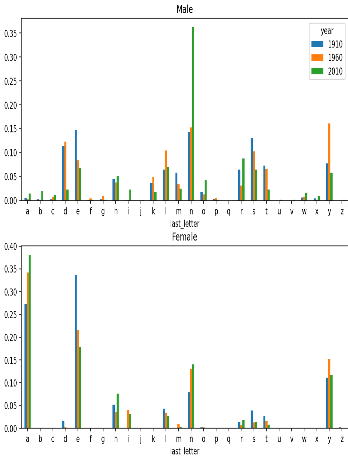
Figure 14-8. Proportion of boy and girl names ending in each letter
