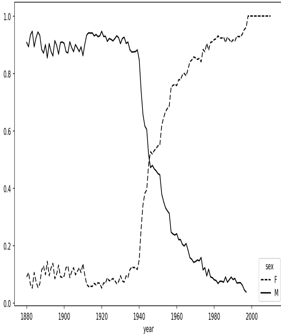
Figure 14-10. Proportion of male/female Lesley-like names over time
