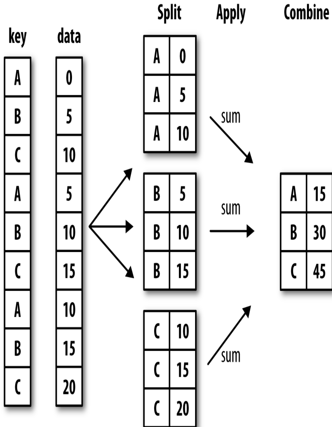
Figure 10-2. Illustration of a group aggregation
