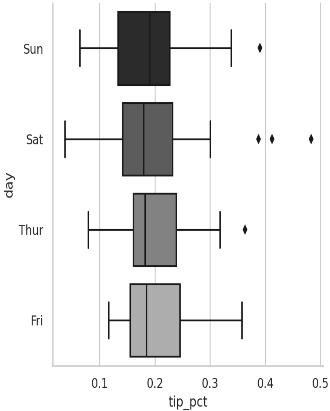
Figure 9-28. Box plot of tip_pct by day
