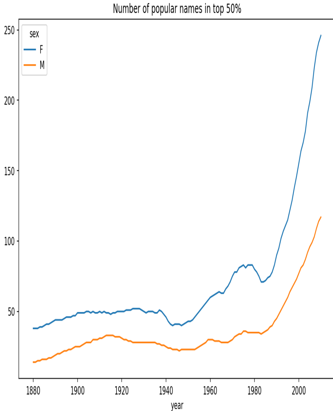
Figure 14-7. Plot of diversity metric by year
