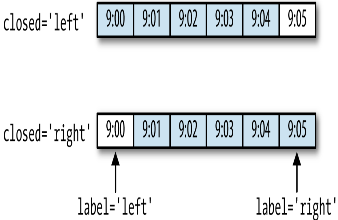
Figure 11-3. Five-minute resampling illustration of closed , label conventions
