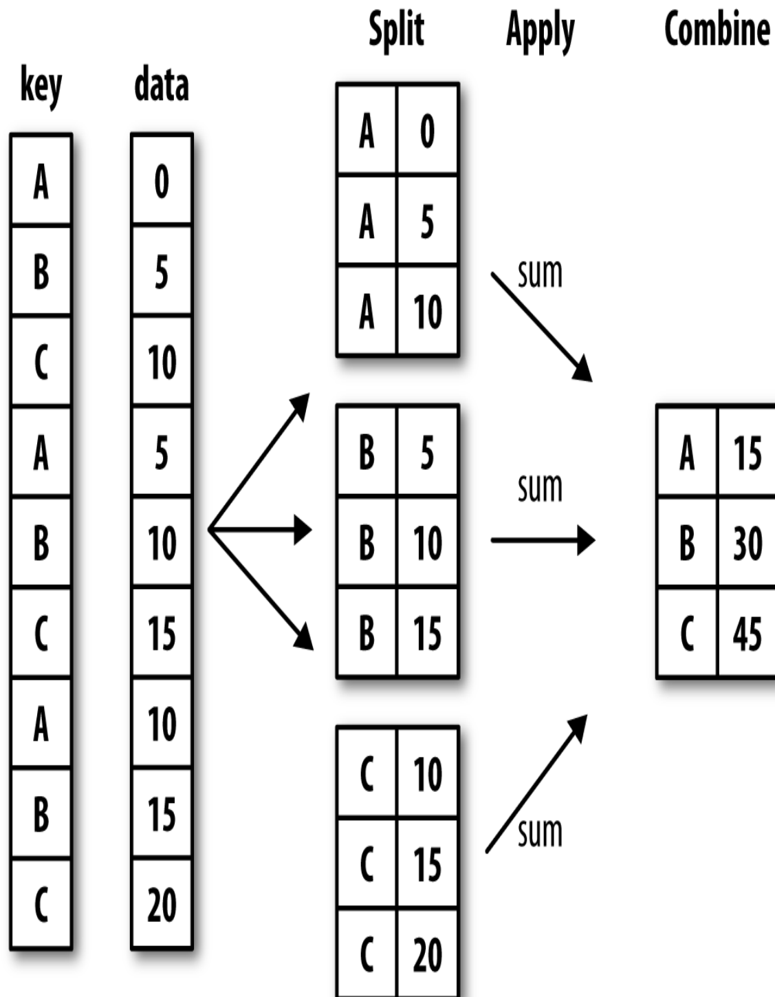
Figure 10-1. Illustration of a group aggregation
