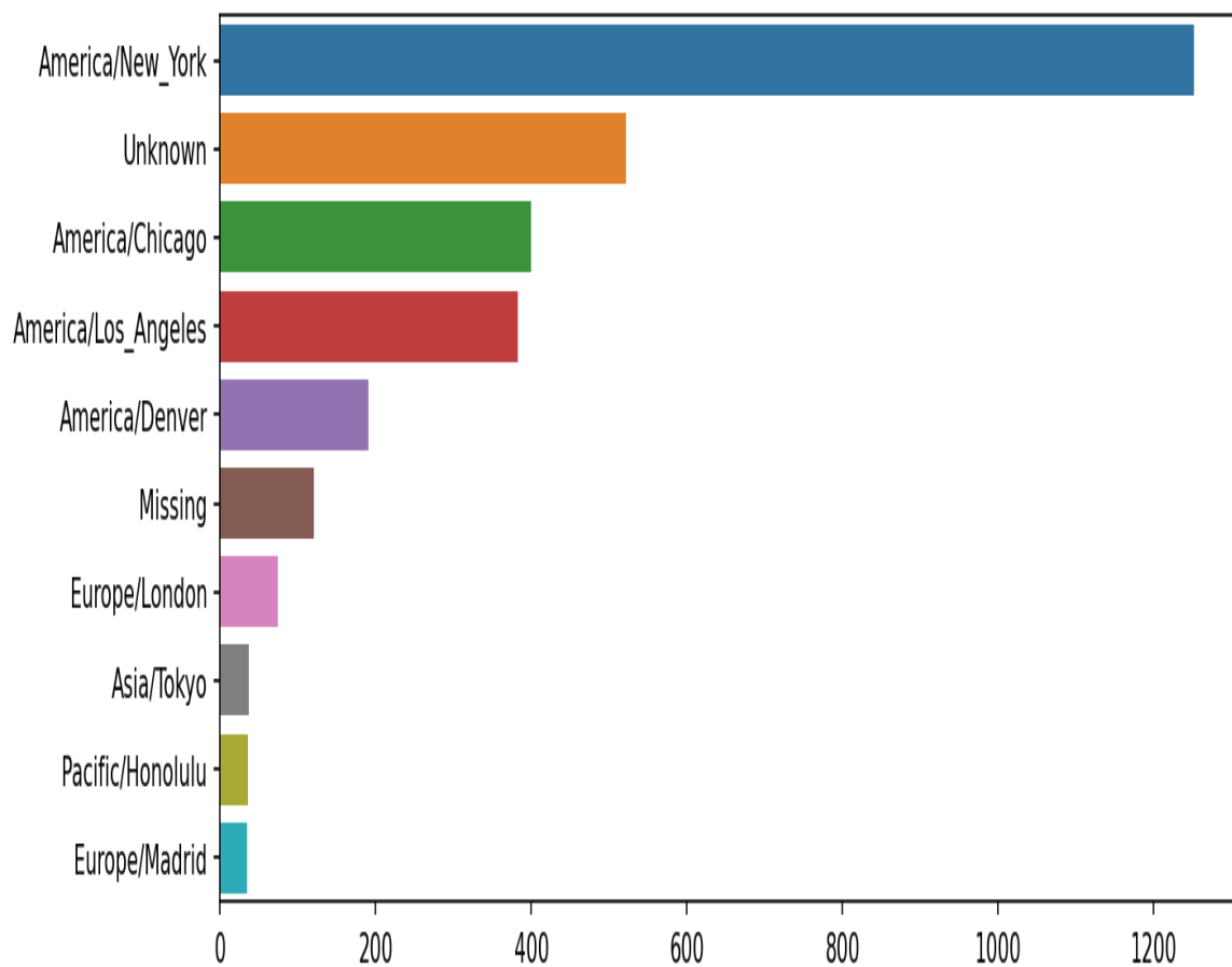
Figure 14-1. Top time zones in the l.usa.gov sample data
