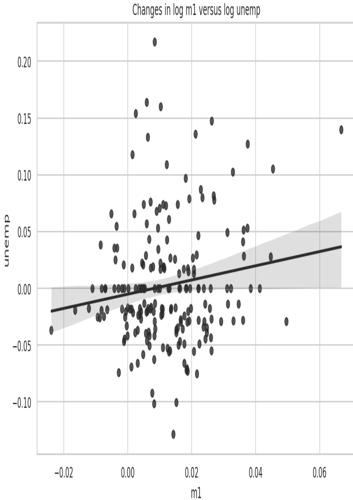
Figure 9-24. A seaborn regression/scatter plot
