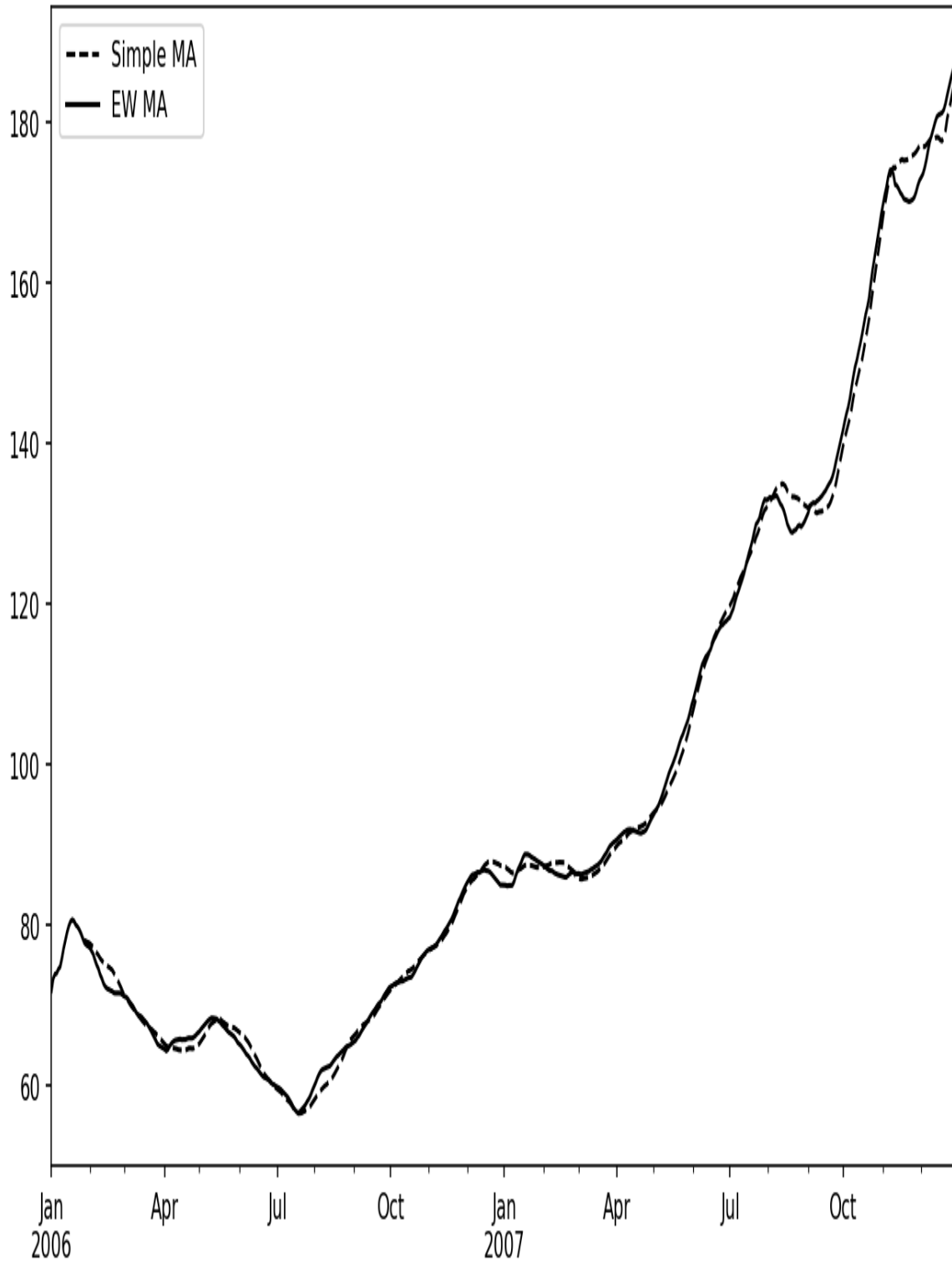
Figure 11-7. Simple moving average versus exponentially weighted
