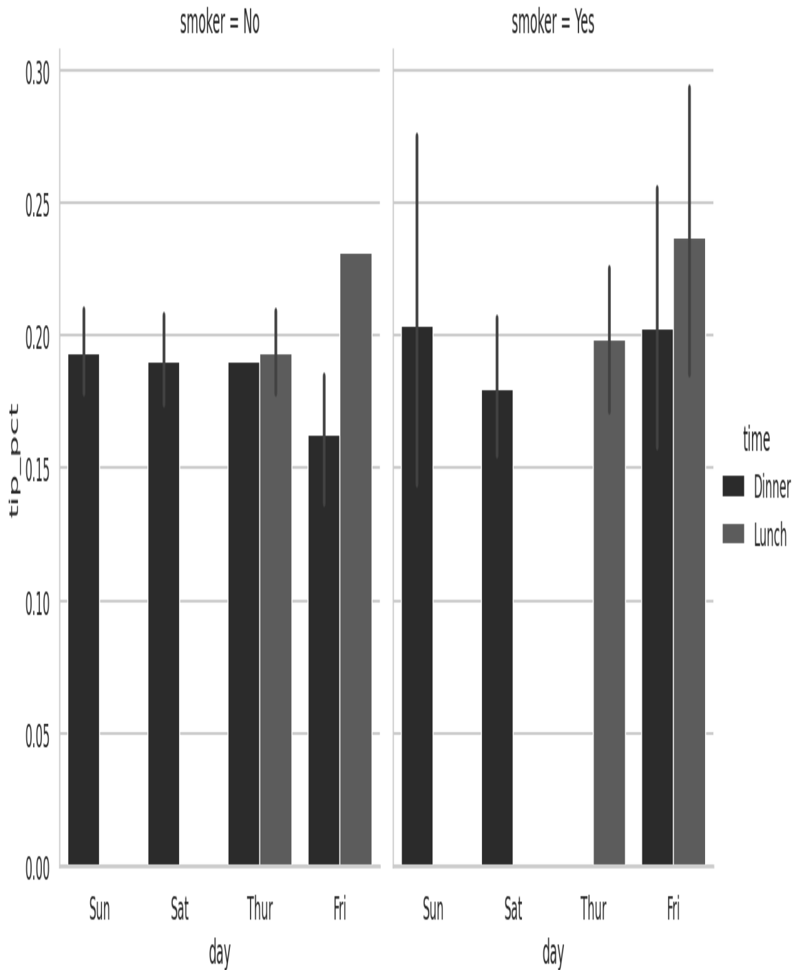
Figure 9-26. Tipping percentage by day/time/smoker
