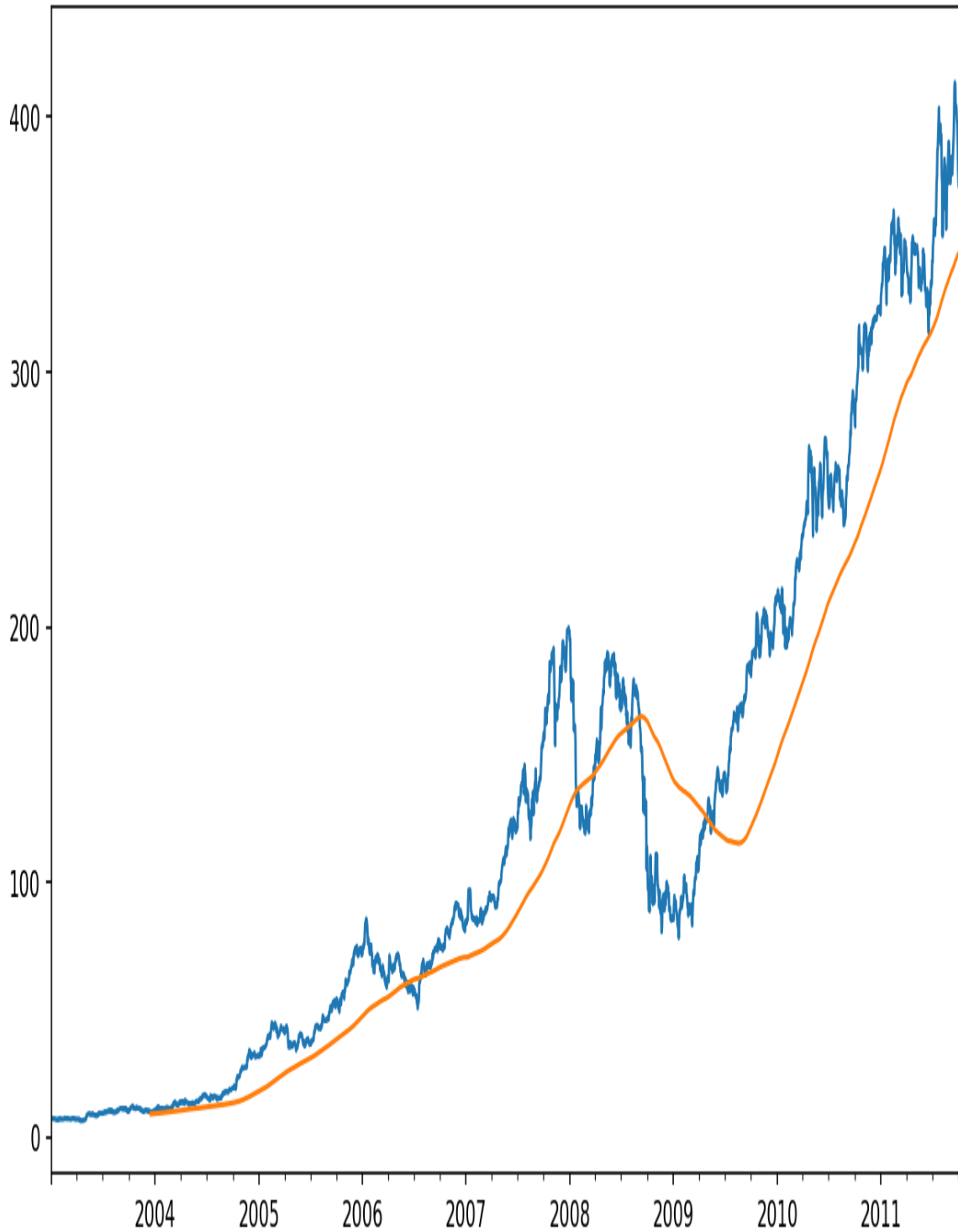
Figure 11-4. Apple Price with 250-day MA
