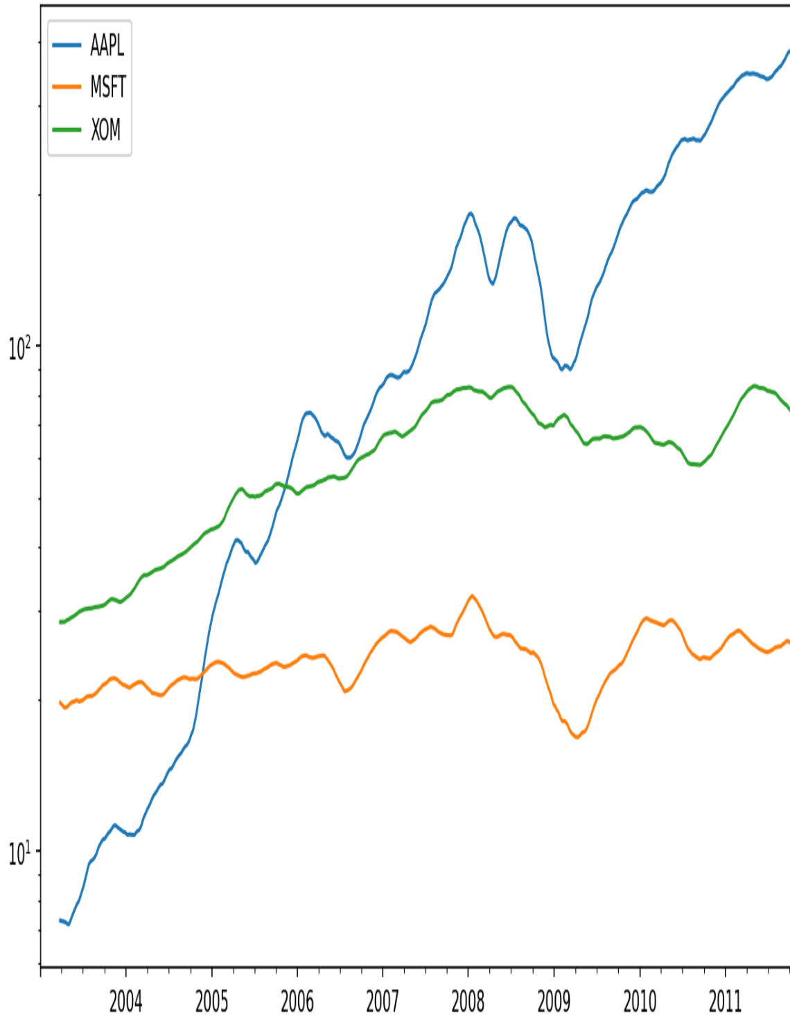
Figure 11-6. Stocks prices 60-day MA (log Y-axis)
