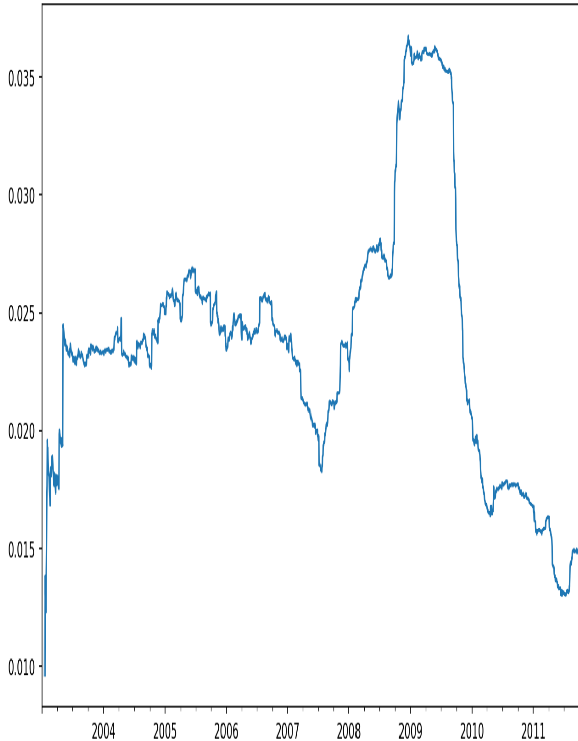
Figure 11-5. Apple 250-day daily return standard deviation
