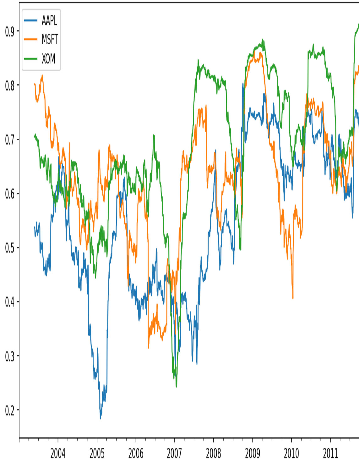
Figure 11-9. Six-month return correlations to S&P 500
