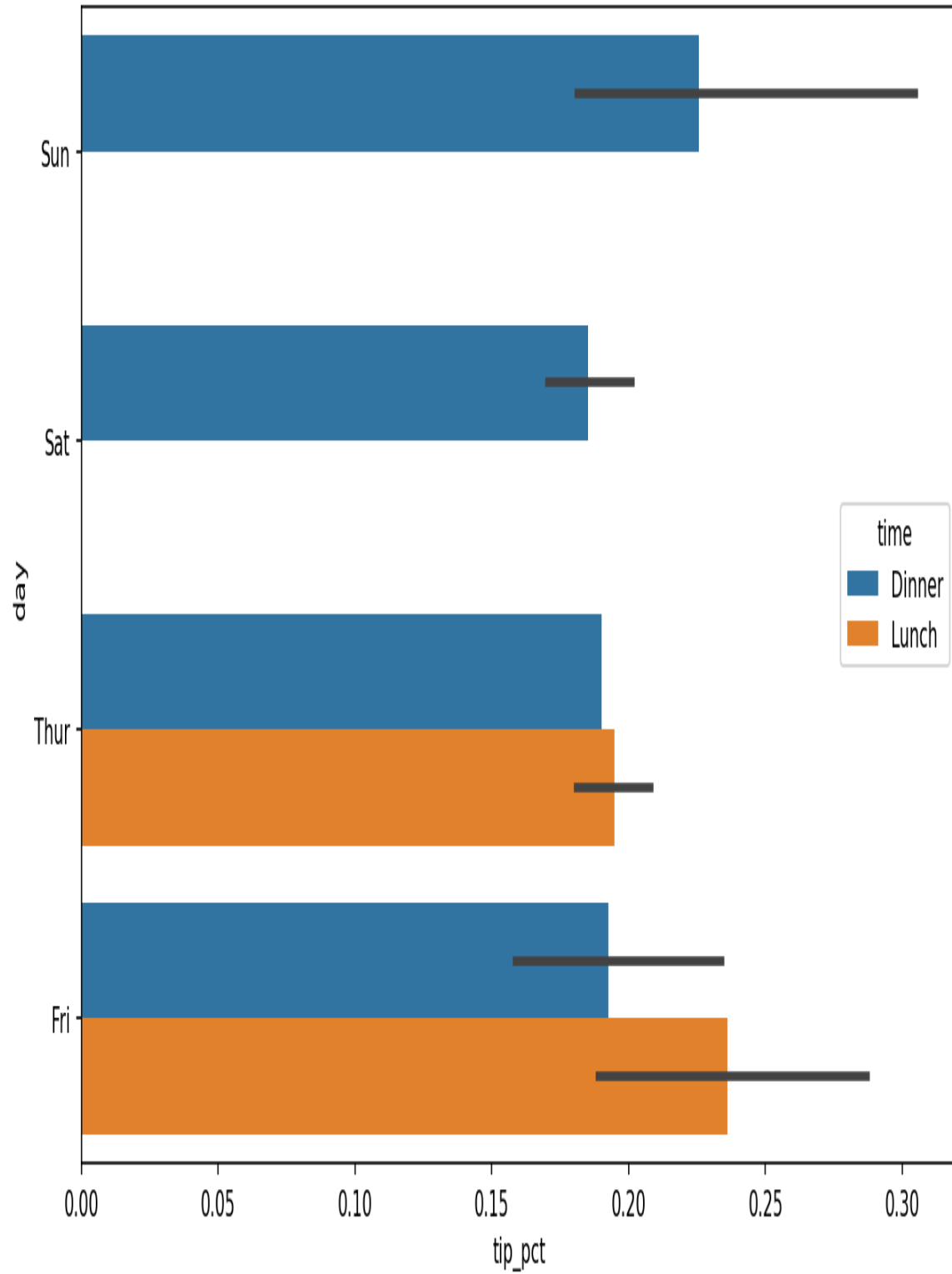
Figure 9-20. Tipping percentage by day and time
