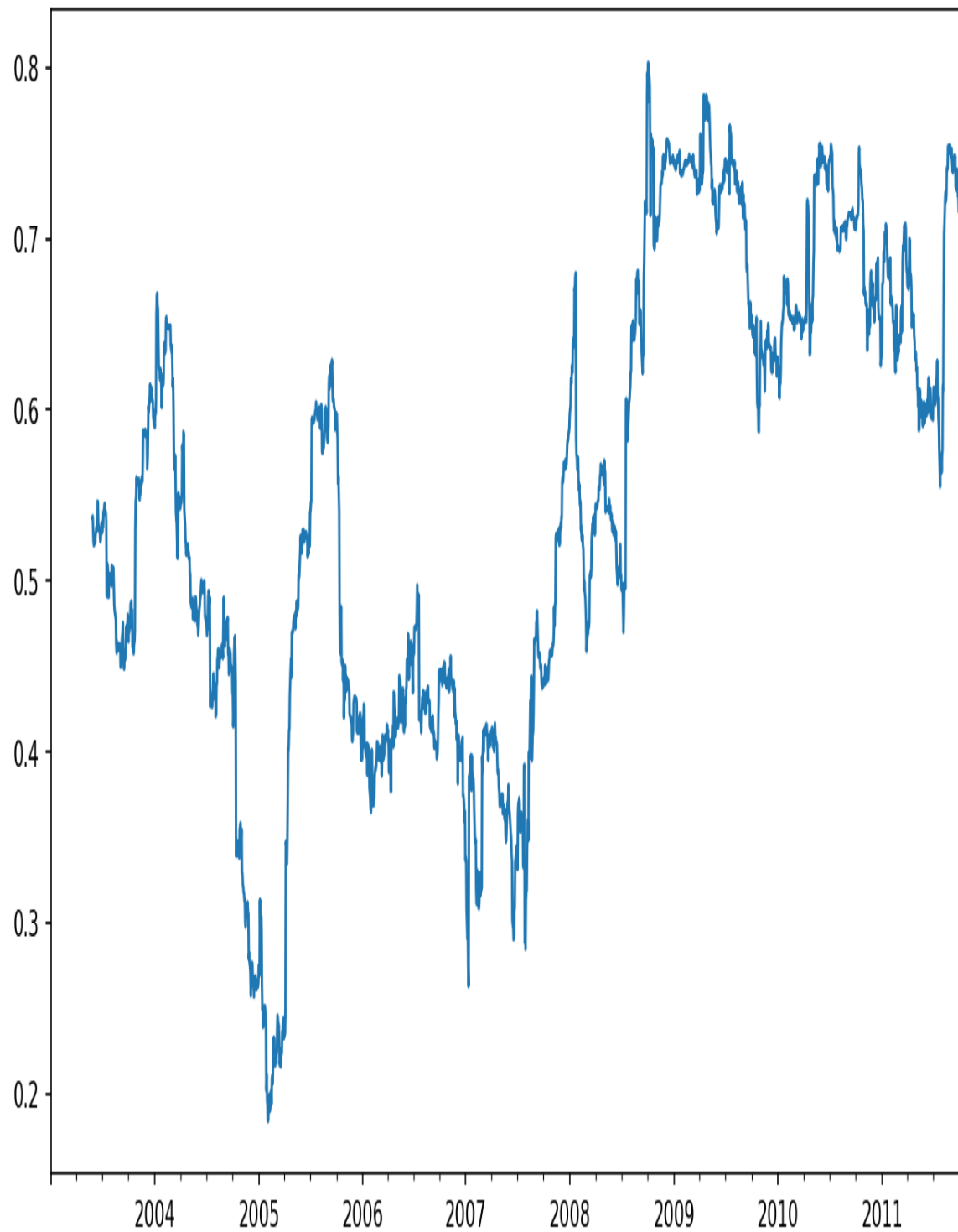
Figure 11-8. Six-month AAPL return correlation to S&P 500
