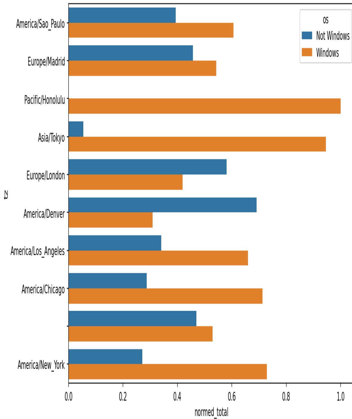
Figure 14-3. Percentage Windows and non-Windows users in top-occurring time zones
