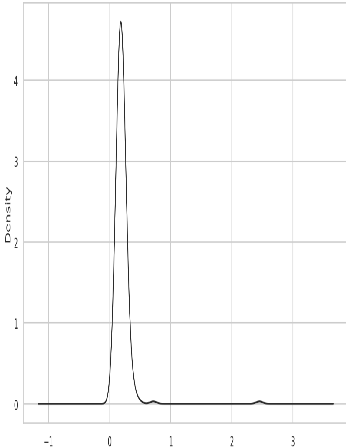
Figure 9-22. Density plot of tip percentages
