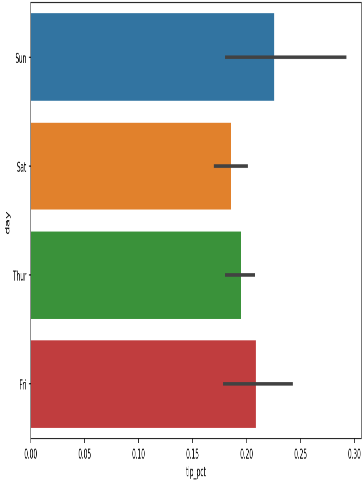
Figure 9-19. Tipping percentage by day with error bars
