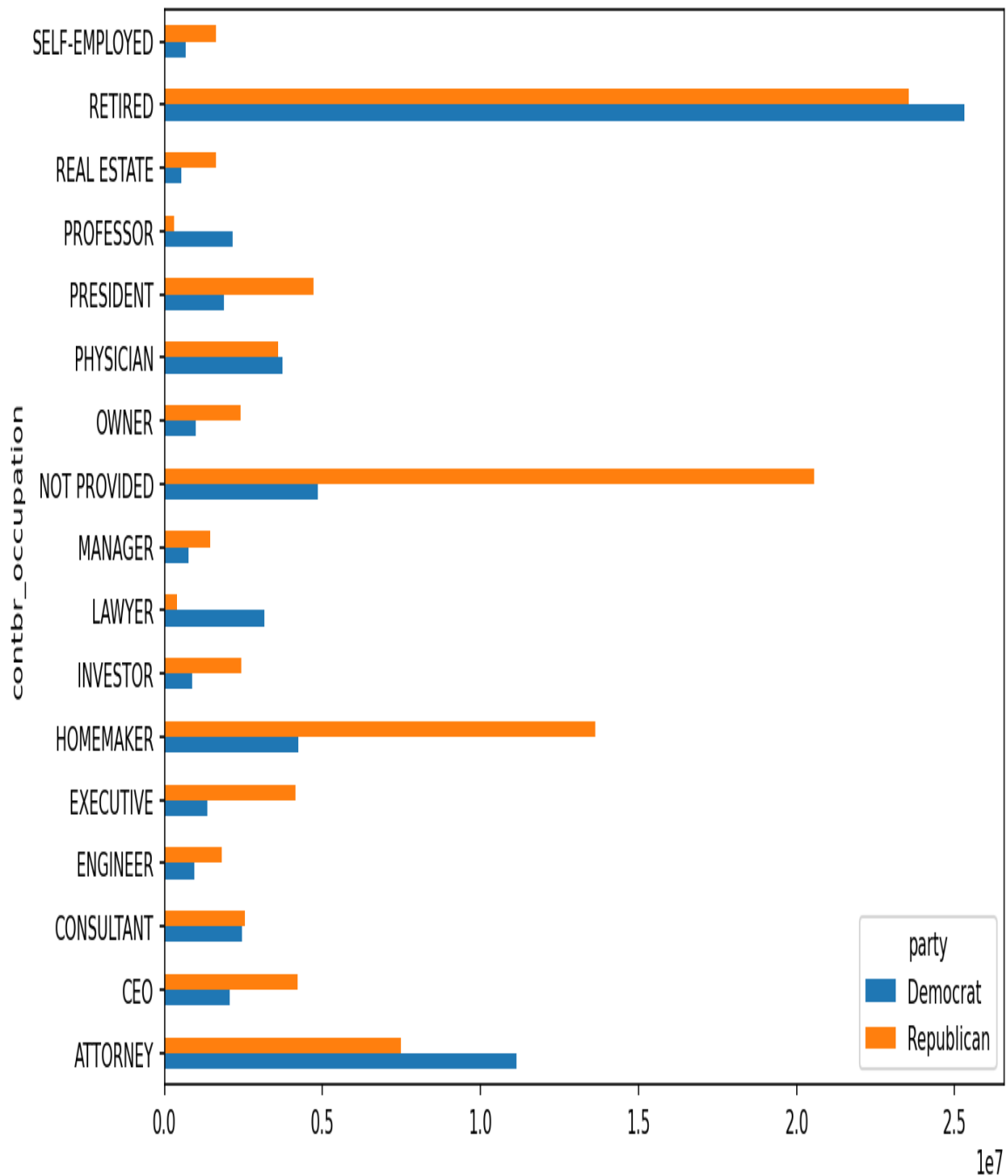
Figure 14-12. Total donations by party for top occupations
