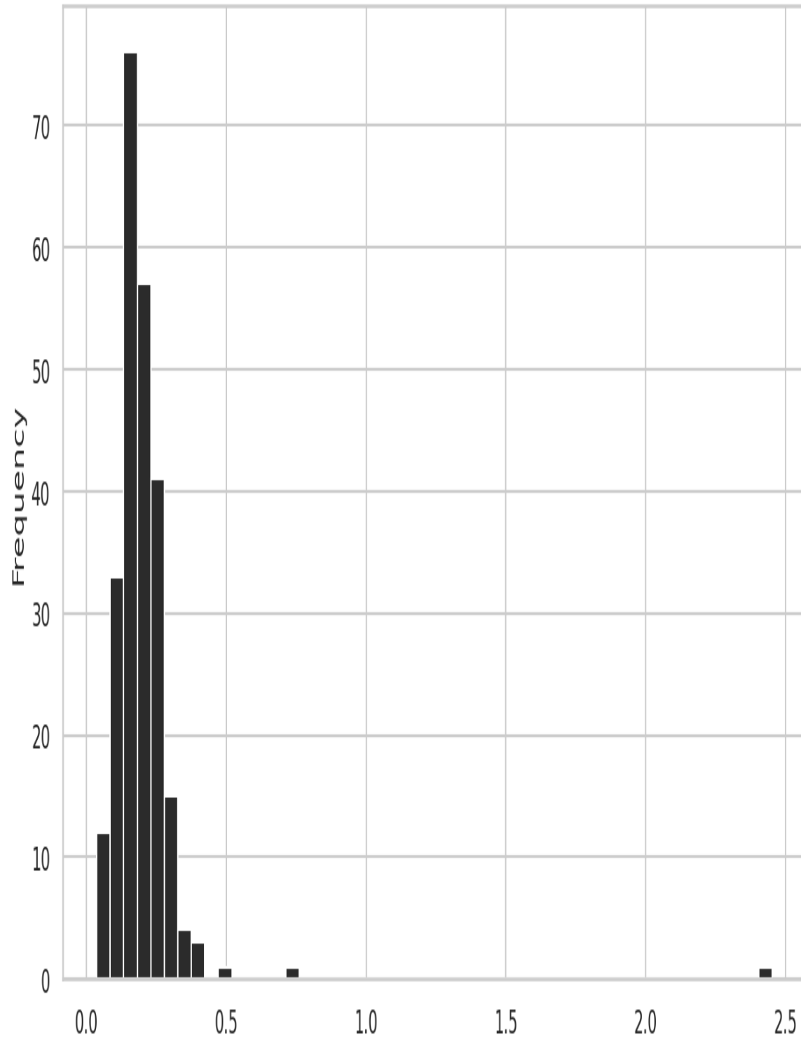
Figure 9-21. Histogram of tip percentages
