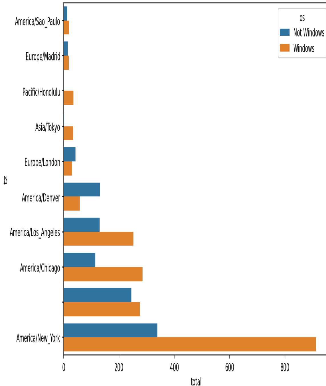
Figure 14-2. Top time zones by Windows and non-Windows users
