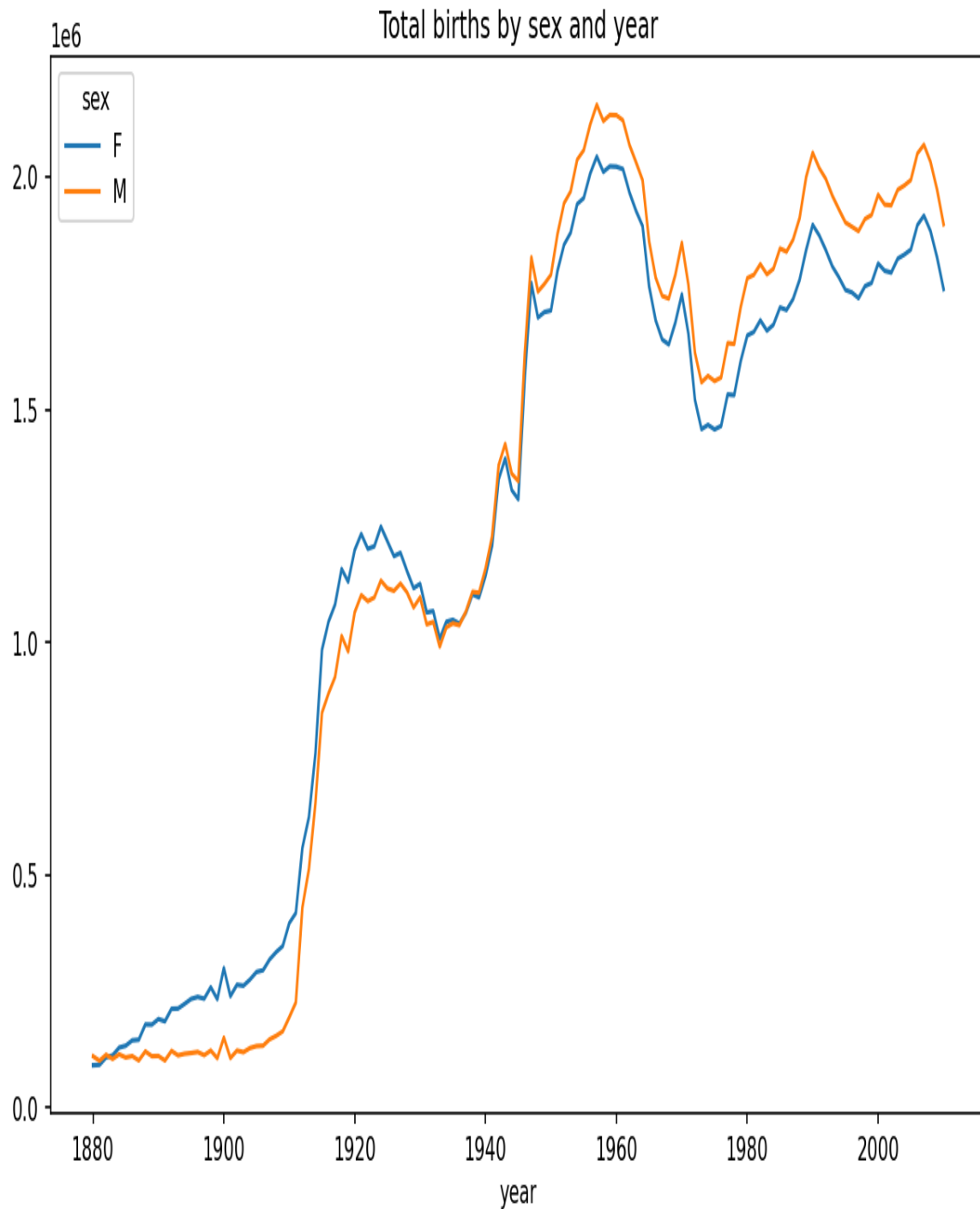
Figure 14-4. Total births by sex and year
