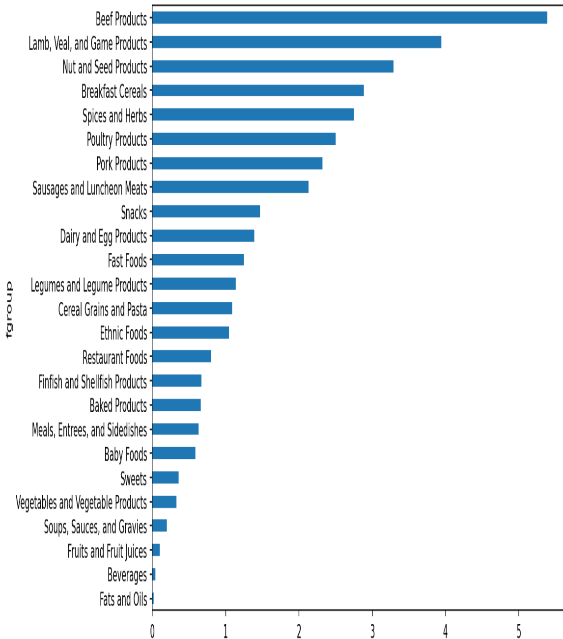
Figure 14-11. Median zinc values by food group
