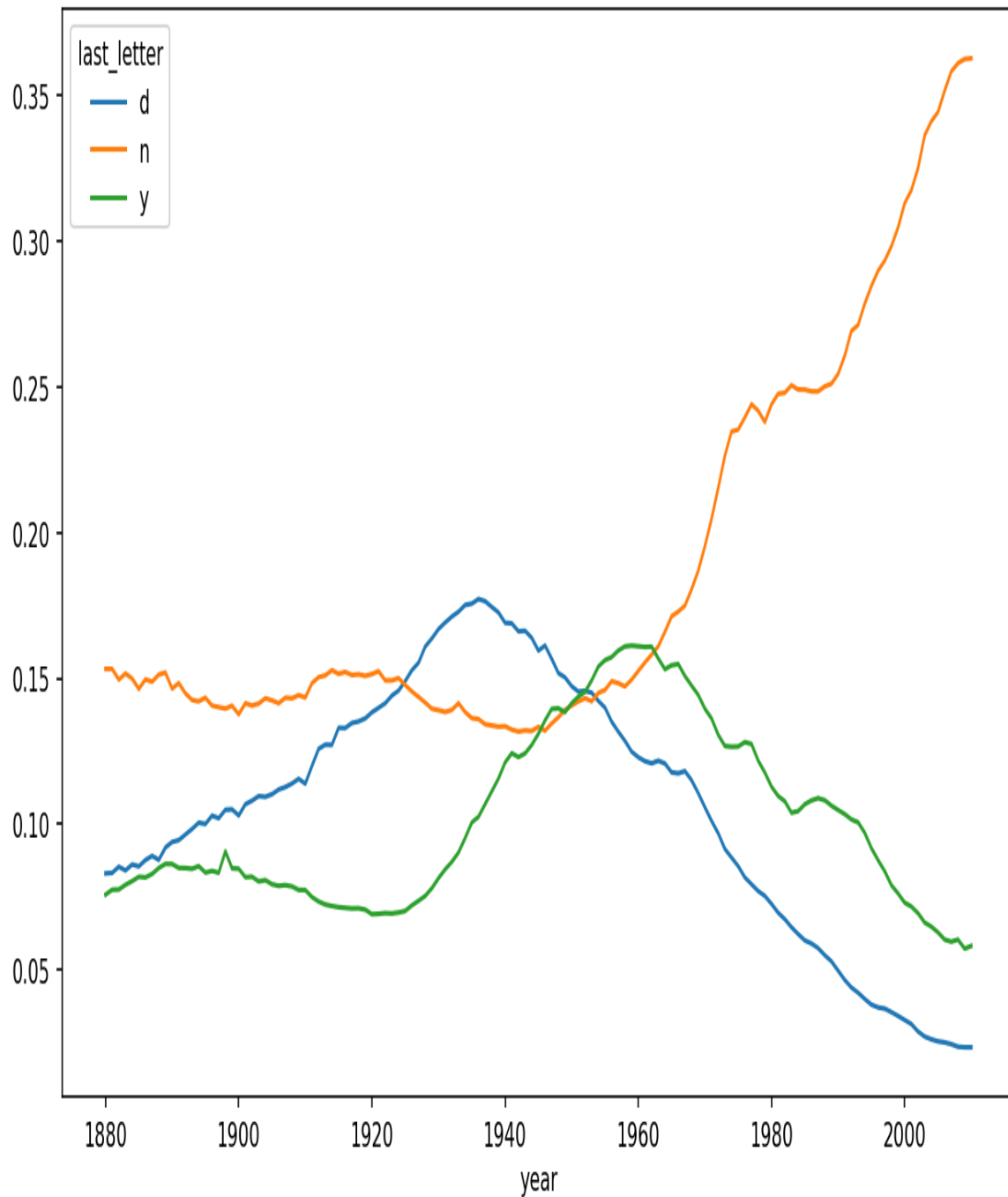
Figure 14-9. Proportion of boys born with names ending in d/n/y over time
