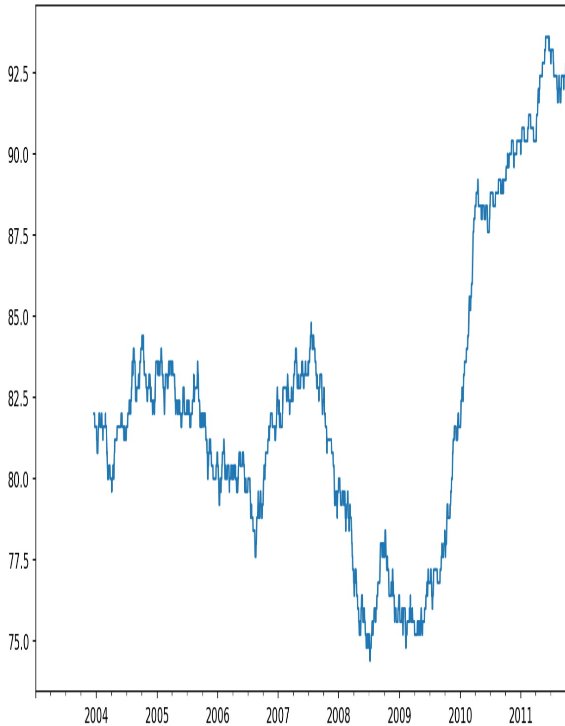
Figure 11-10. Percentile rank of 2% AAPL return over one-year window
